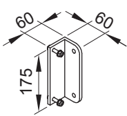
angled bracket for lateral face fixture 77822. 175 × 60 × 60 mm
