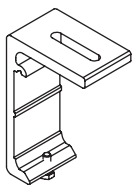
cassette bracket for reveal fixture 50 mm
