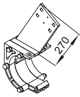
eaves fixture bracket 150 mm, 5°-35° height of flat plate 270 mm
