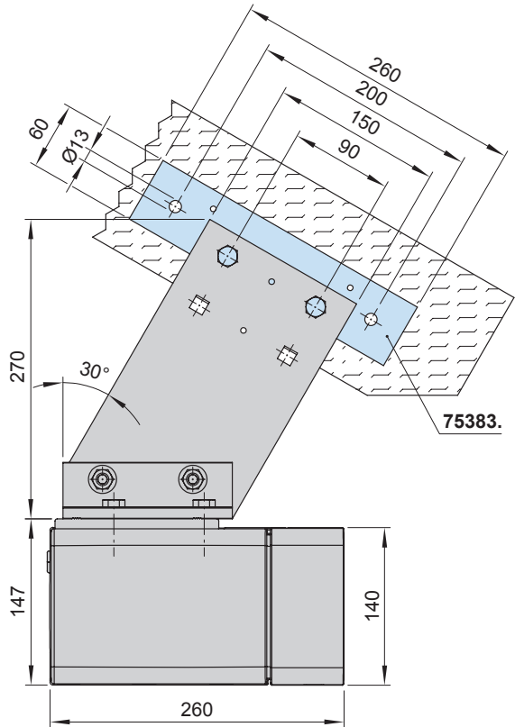
Eaves fixture bracket with backing plate for 71659.
